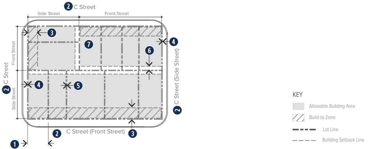
Figure 660-20(2) Lane Rowhouse Siting
