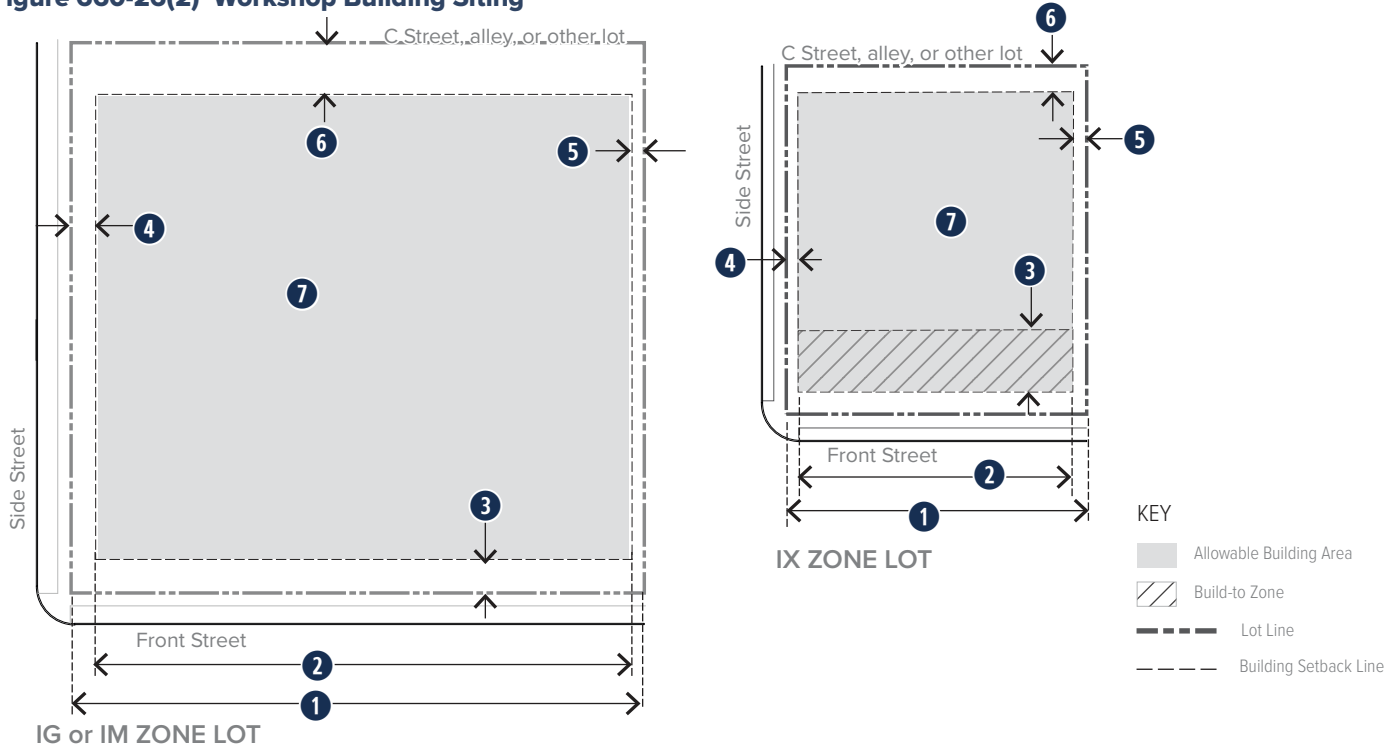
Figure 660-26(2) Workshop Building Siting
