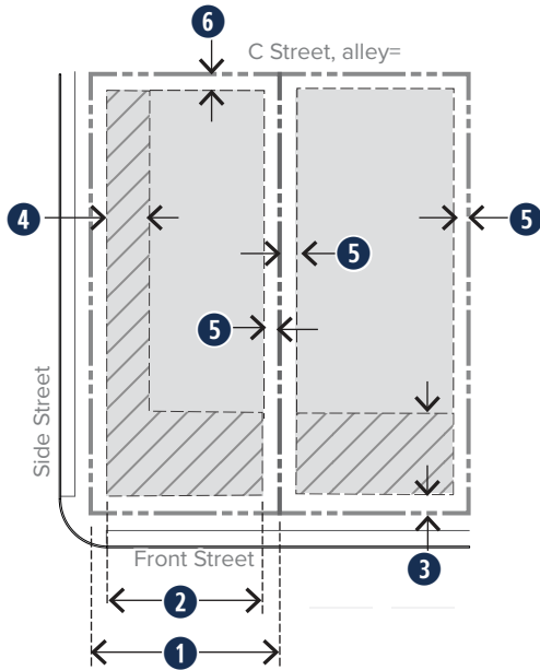
Figure 660-17(2) Small General Building Siting
