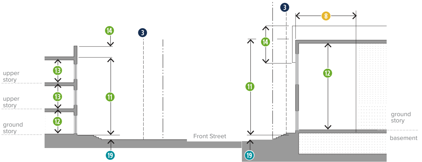
Figure 660-27(4) Civic Building Height and Roofs
