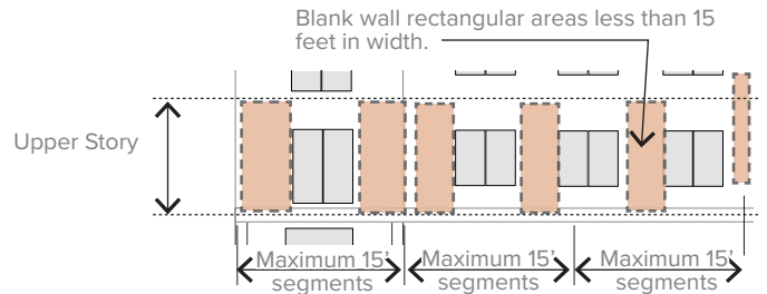
Figure 660(42) Blank Wall Segments (2)
