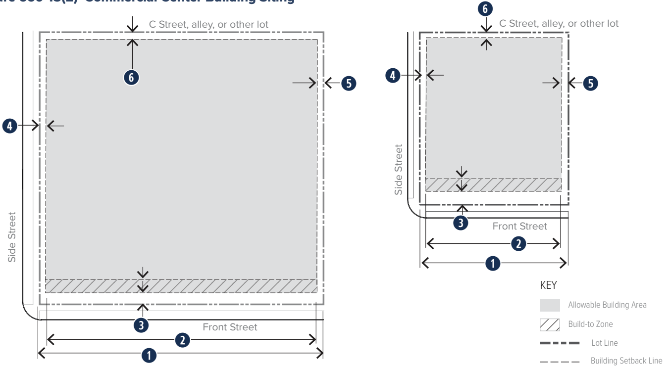
Figure 660-15(2) Commercial Center Building Siting
