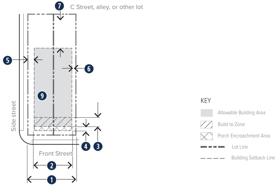
Figure 660-22(2) Twin House Siting
