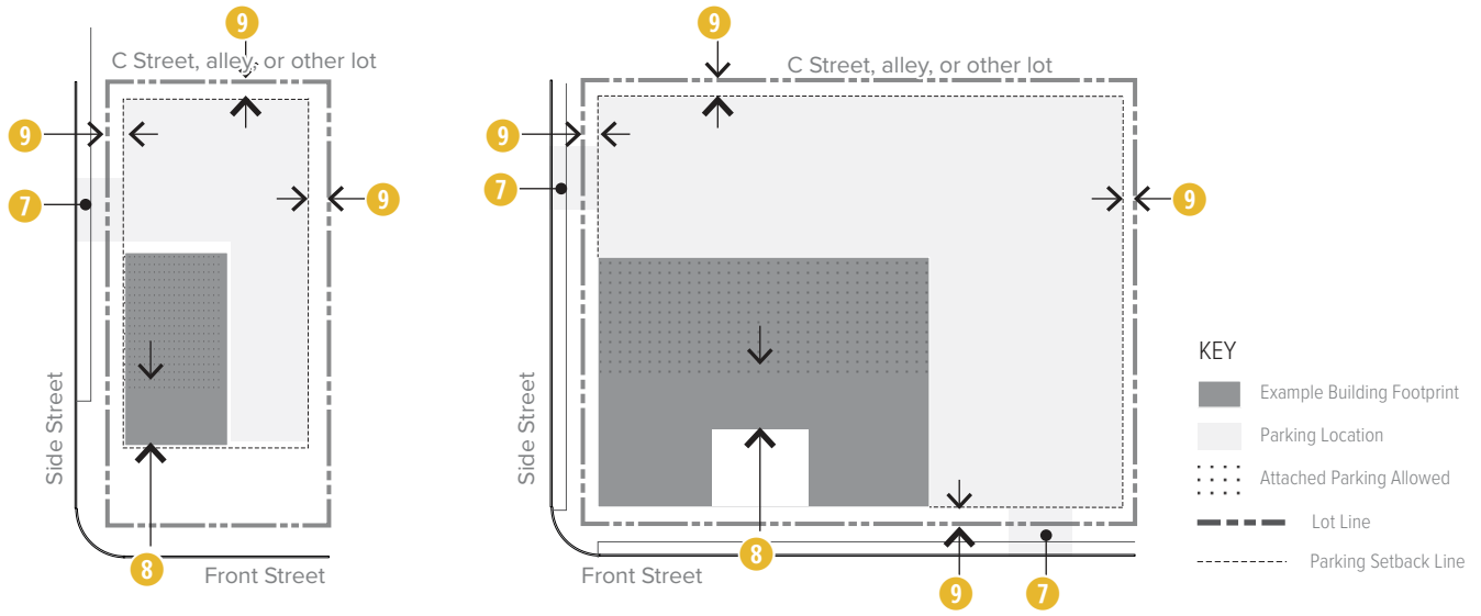
Figure 660-27(3) Civic Building Parking Siting
