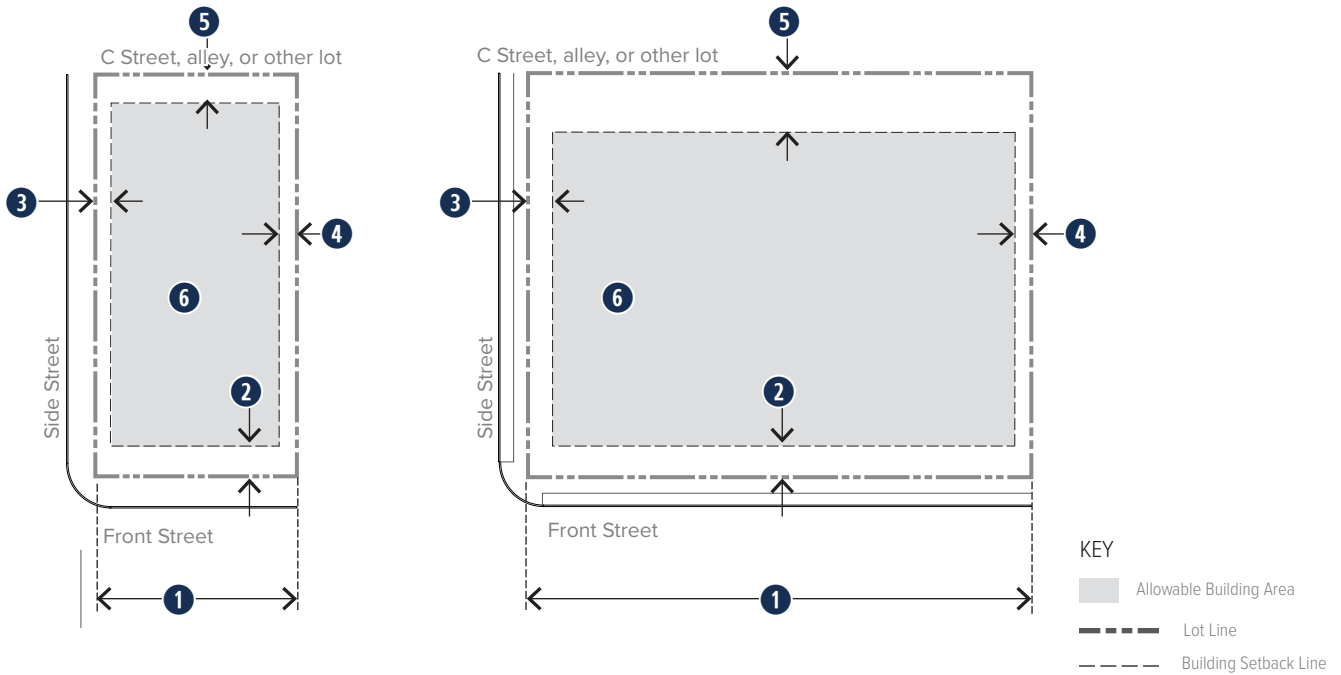
Figure 660-27(2) Civic Building Siting
