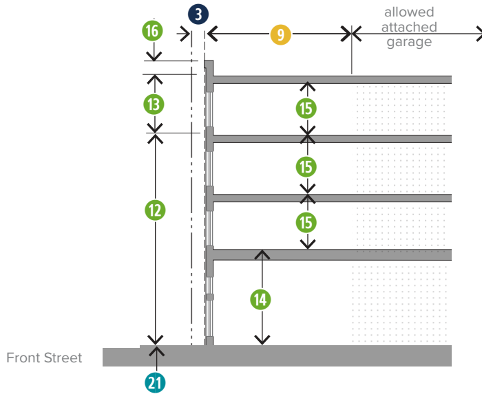
Figure 660-14(4) Storefront Building Height and Roofs
