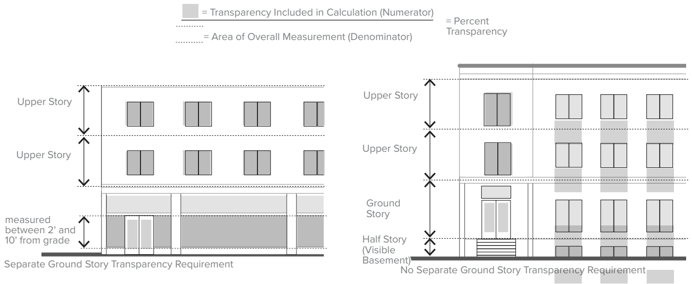
Figure 660(40) Measuring Transparency Floor-to-Floor
