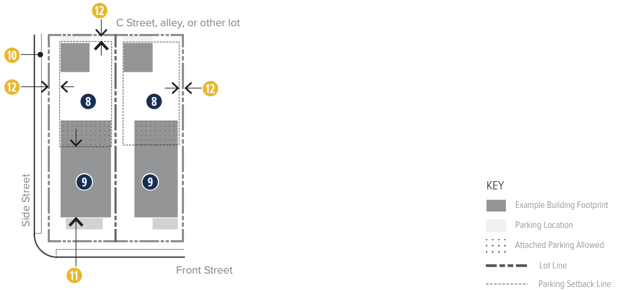
Figure 660-23(3) House A Parking Siting
