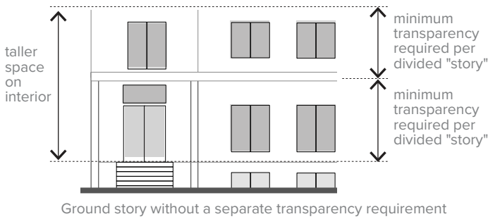
Figure 660(41) Blank Wall Segments (1)
