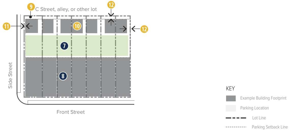
Figure 660-19(3) Urban Rowhouse Parking Siting
