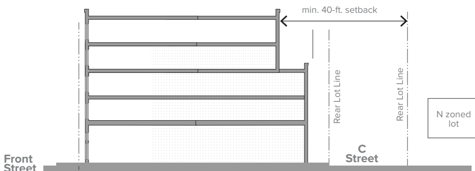
Figure 660-14(6) Required Setback Additional Height along Mixed-Use Corridors across from N Zone
