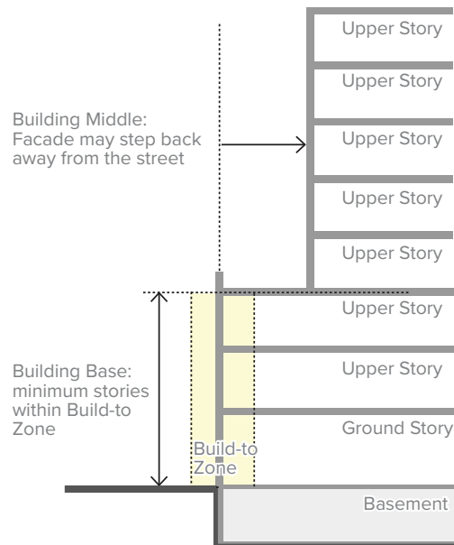
Figure 660(20) Building Massing in Build-to Zone
