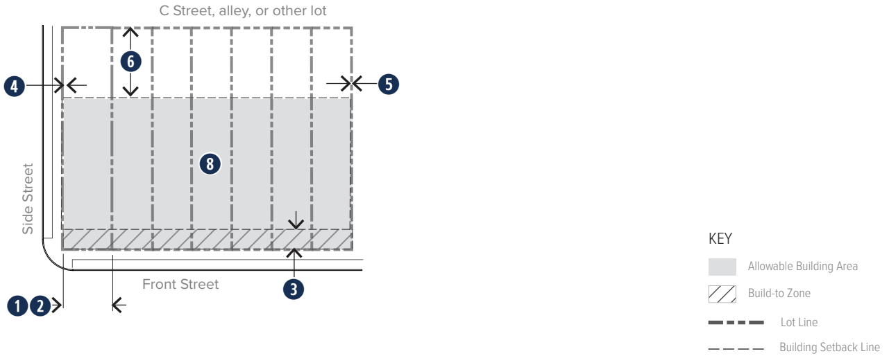
Figure 660-19(2) Urban Rowhouse Siting
